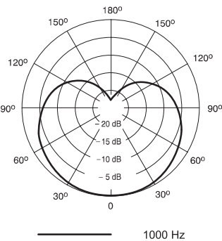
Polar Pattern
