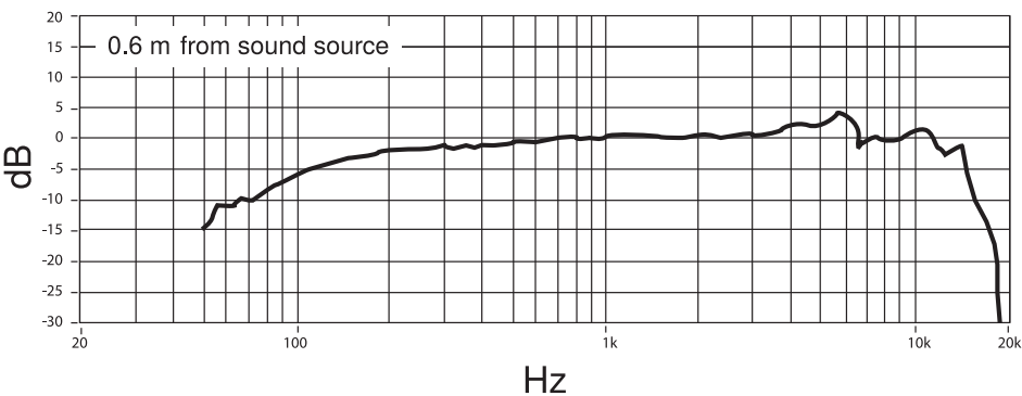
Frequency Response
