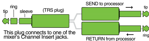
Unbalanced 1/4" Insert Connectors
