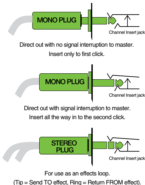
Using the Send Only on an Insert Jack
