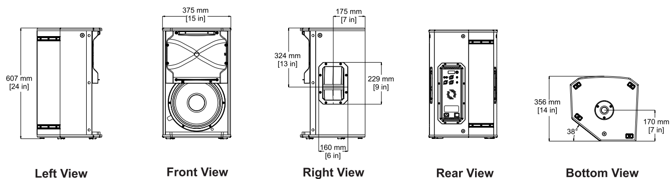
Figure 3.1: EKV-12P dimensions
